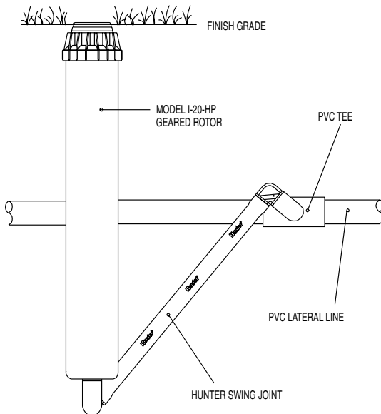
Hunter® I-20-HP
