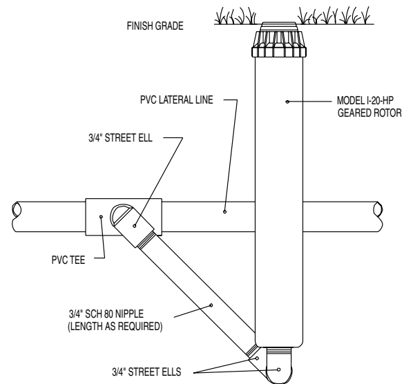
Hunter® I-20-HP
