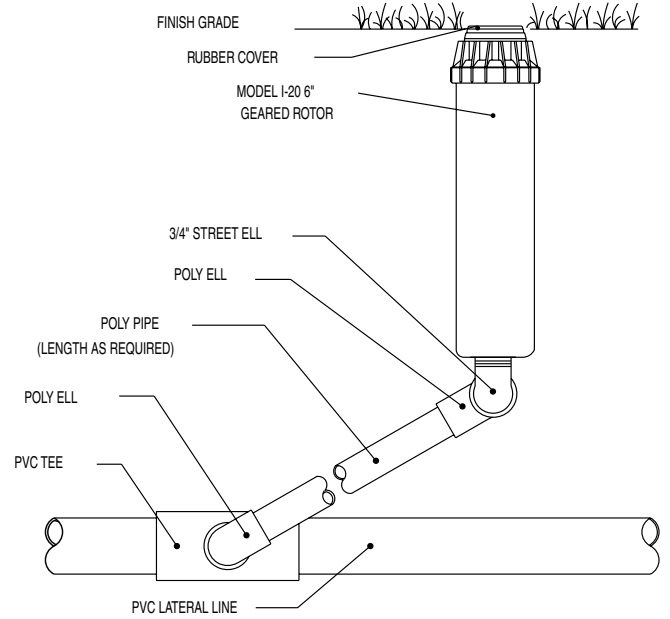
Hunter® I-20-6P
